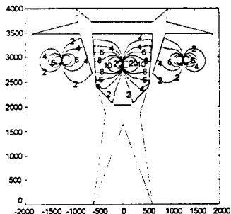
(b) Equigradient contours (horizontal component) without tower and with tower; V_{\text{left}} = +50 \text{ V} , V_{\text{center}} = -100 \text{ V} , V_{\text{right}} = +50 \text{ V} .
