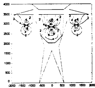
(c) Equigradient contours (vertical component) without tower and with tower; V_{\text{left}} = +50 \text{ V} , V_{\text{center}} = -100 \text{ V} , V_{\text{right}} = +50 \text{ V} .
