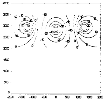
(a) Equipotential contours of conductors without tower; V_{left} = +50 V, V_{center} = -100 V, V_{right} = +50 V.
