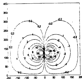
(b) Equipotential contours of horizontal sphere gap, V_{left} = +50 \text{ V} , V_{right} = -50 \text{ V} .
