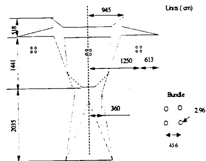
Figure 2. Simplified geometry and major dimensions of the power line tower and conductors.
