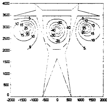
(b) Equipotential contours of conductors with tower; V_{left} = +50 V, V_{center} = -100 V, V_{right} = +50 V.
