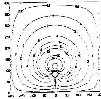
(c) Equipotential contours of vertical sphere gap, V_{up} = +100 \text{ V} , V_{down} = 0 \text{ V} .
