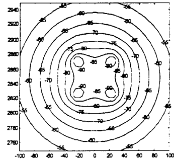
(c) The enlarged view of the equipotential contours around the center phase conductors in the tower window; V_{left} = +50 V, V_{center} = -100 V, V_{right} = +50 V.
