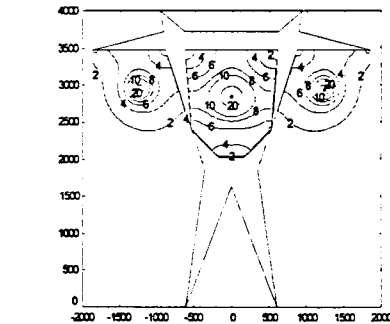
(a) Equigradient contours (magnitude) without tower and with tower; V_{left} = +50 V, V_{center} = -100 V, V_{right} = +50 V.
