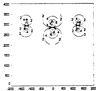
(b) Equigradient contours (horizontal component) without tower and with tower; V_{\text{left}} = +50 \text{ V} , V_{\text{center}} = -100 \text{ V} , V_{\text{right}} = +50 \text{ V} .
