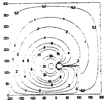
(a) Equipotential contours of horizontal sphere gap, V_{left} = +100 \text{ V} , V_{right} = 0 \text{ V} .
